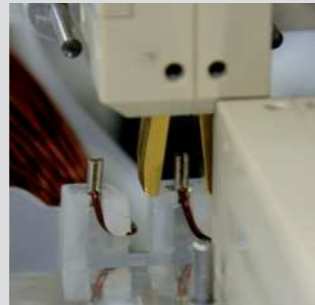
Contacting of contact pins with Kelvin clamps
